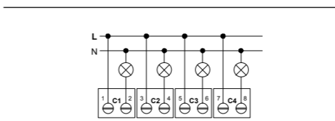
e Connection loads EK-FA1-TP (4-fold)
